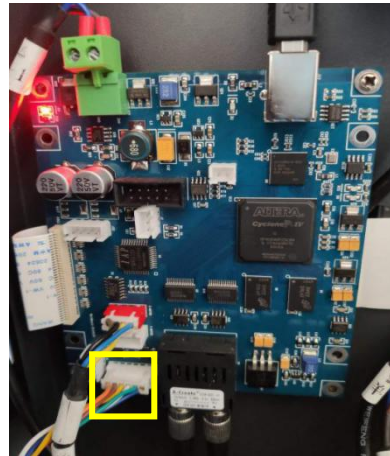
J29 Control panel port on mainboard
